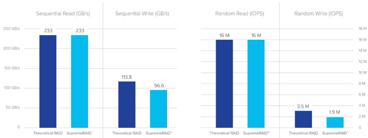
Figure 3: SupremeRAID™ Performance Results vs. Theoretical RAID
